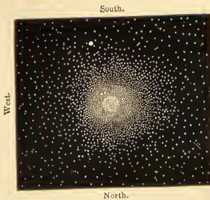
FIG. 43.—Some clusters and nebulae.
